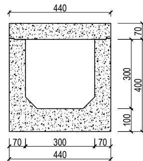
POT. U-DITCH
