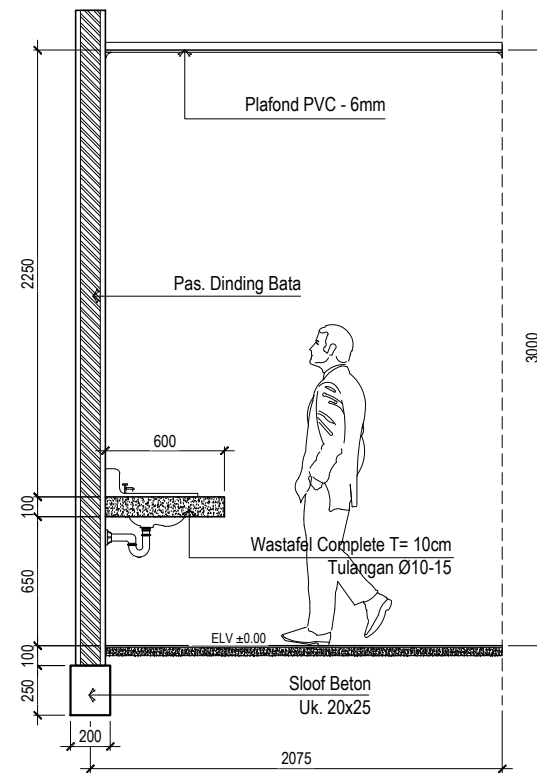
GSG ARS 1:35 DETAIL POTONGAN B-B
