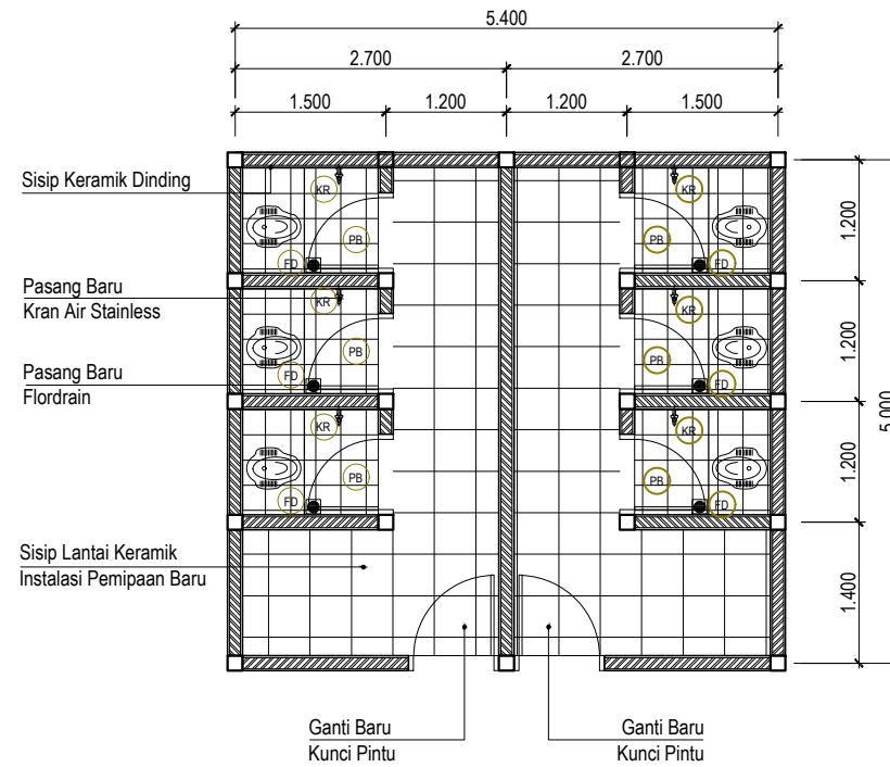
GSG ARS 1:75 DENAH REHAB TOILET D
