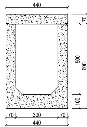
POT. U-DITCH
