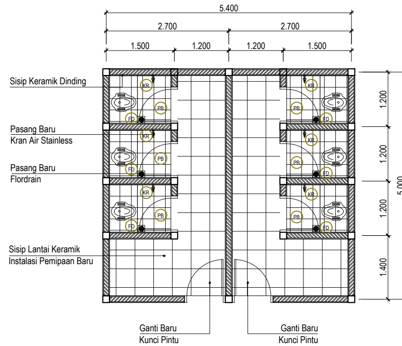
GSG ARS 1:75 DENAH REHAB TOILET B
