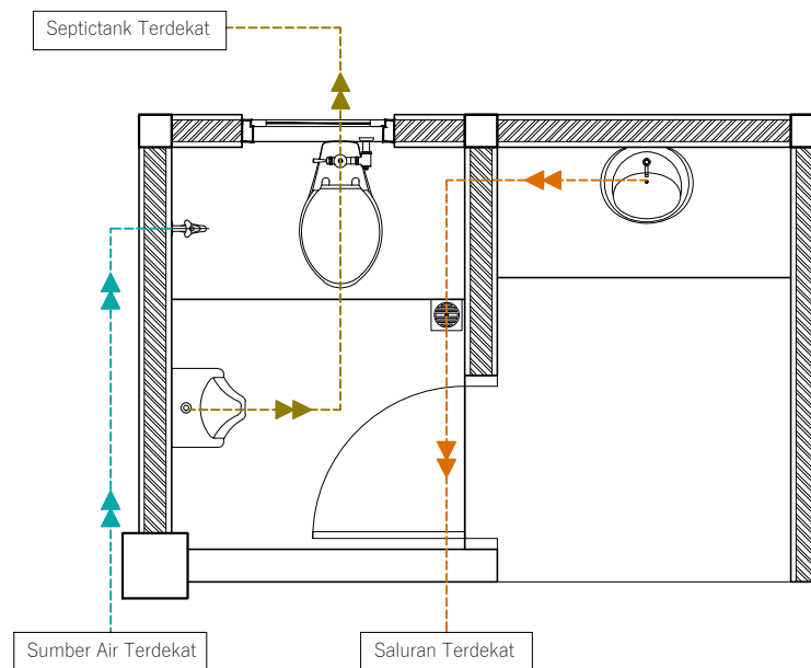
GSG ARS 1:35 DENAH INSTALASI MEKANIKAL
