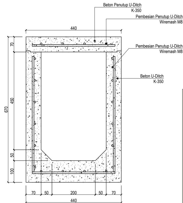
POT. U-DITCH
