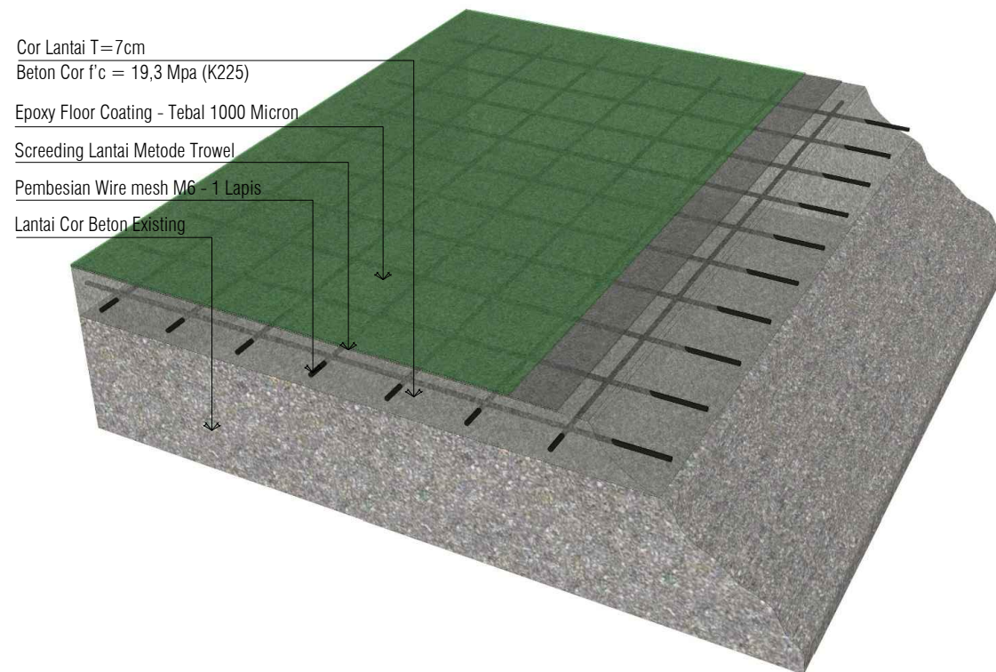
GSG ARS 1:5 DETAIL 3D LANTAI BASEMANT
