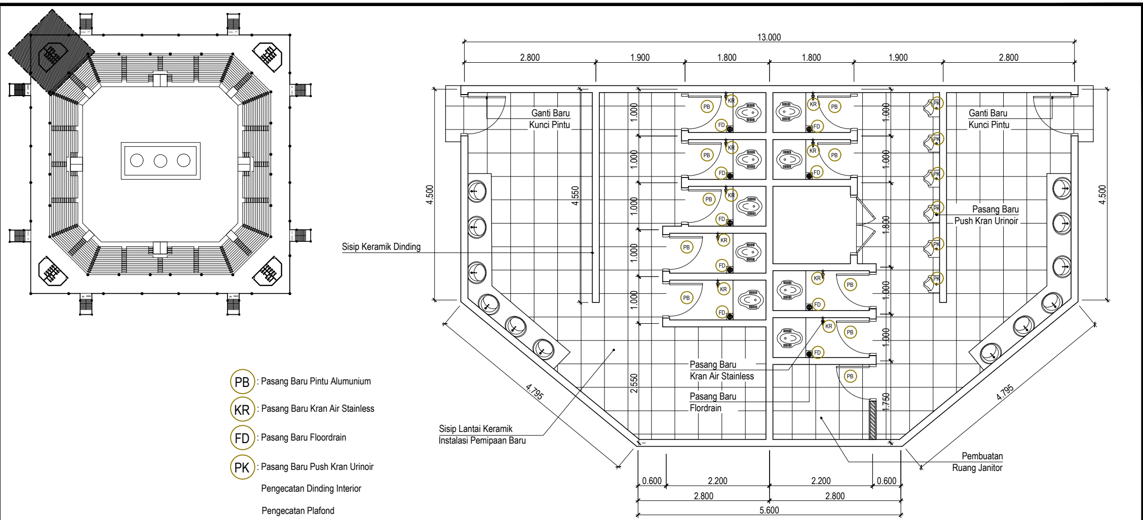
GSG ARS 1: 75 DENAH RENCANA REHAB TOILET A
