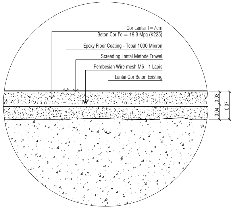
GSG ARS 1:5 DETAIL LANTAI BASEMANT
