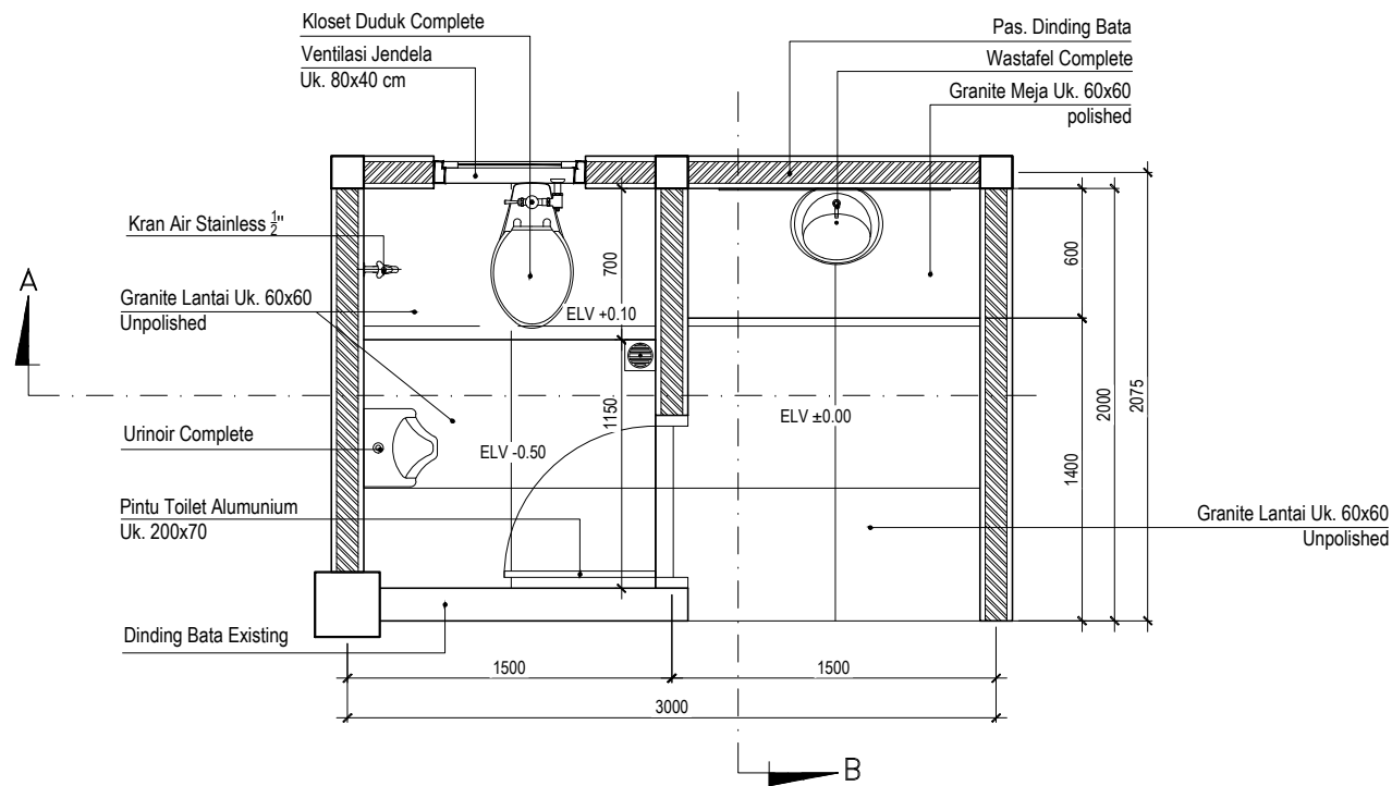
GSG ARS 1:35 DENAH TOILET PDBI
