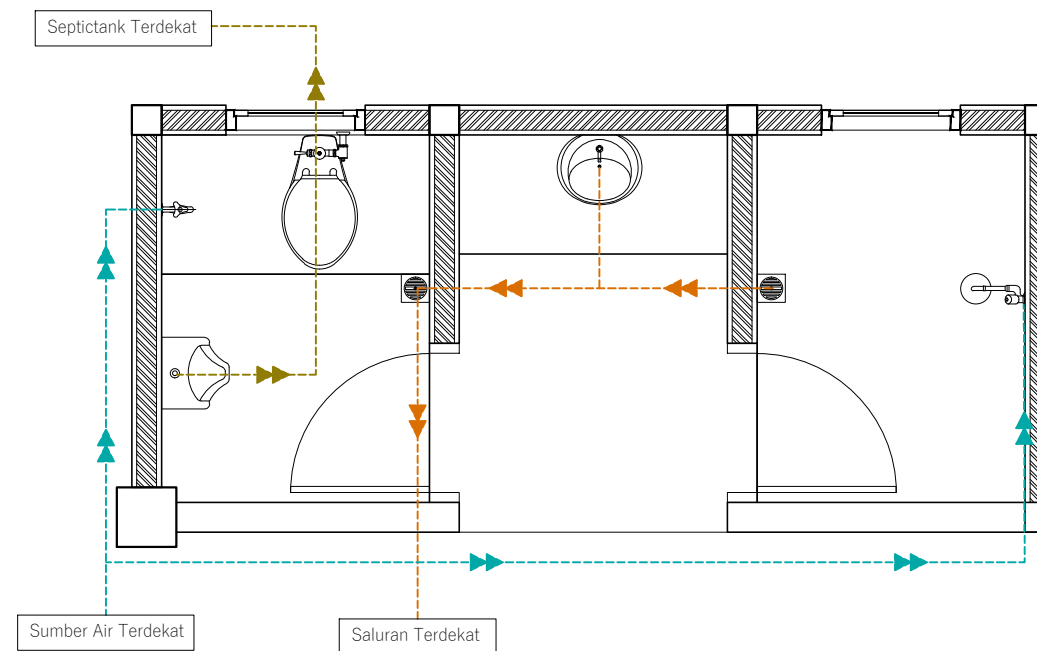
GSG ARS 1:35 DENAH INSTALASI MEKANIKAL
