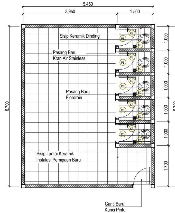
GSG ARS 1:75 DENAH REHAB TOILET C
