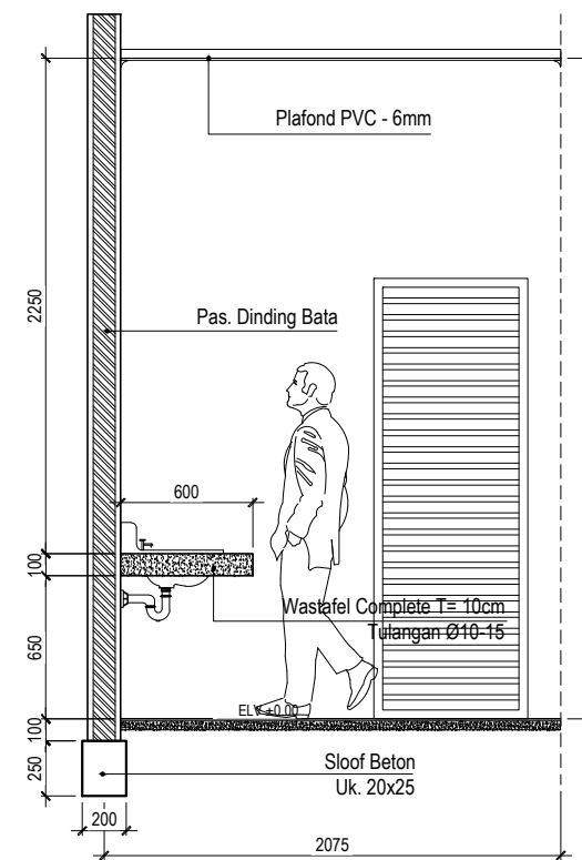
GSG ARS 1:35 DETAIL POTONGAN B-B
