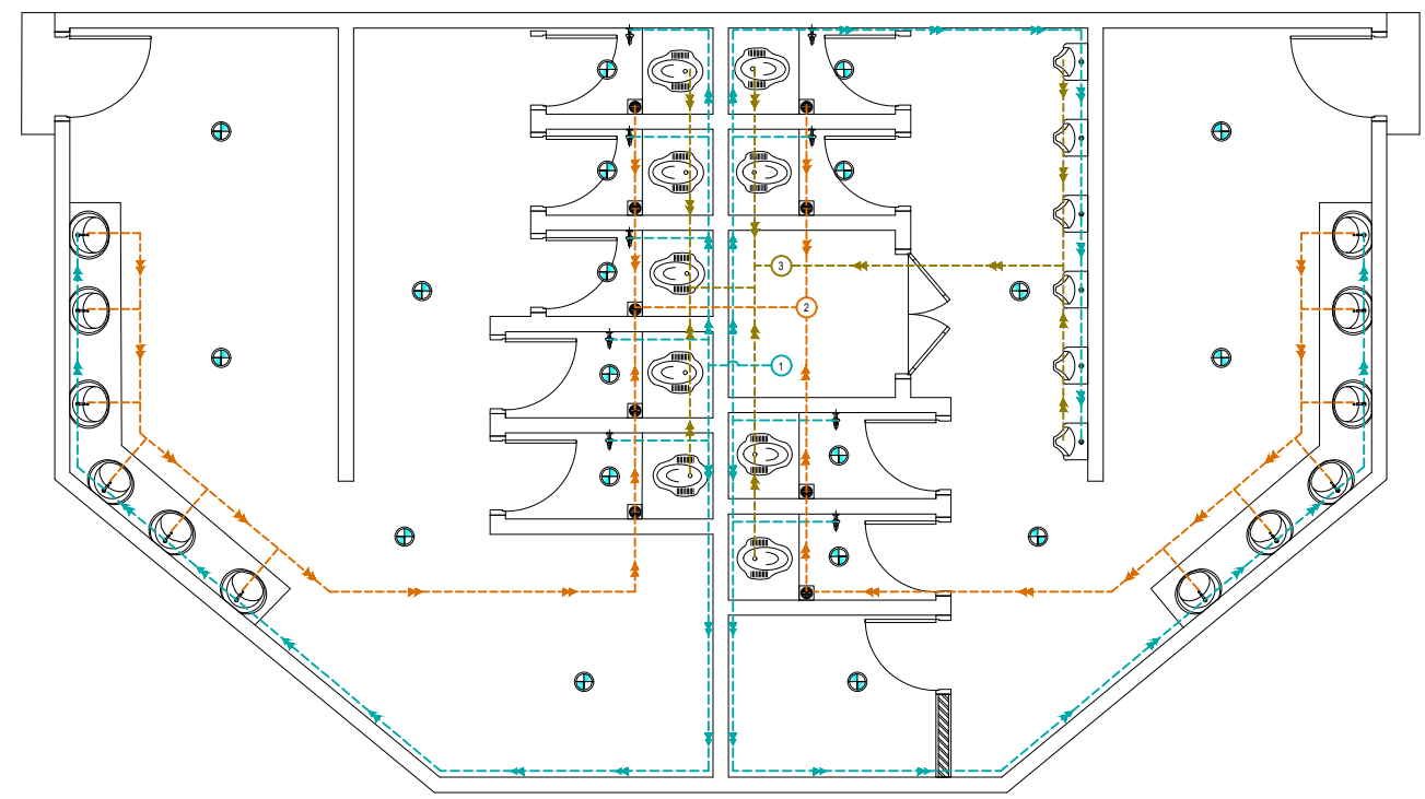
DENAH INSTALASI MEKANIKAL & ELEKTRIKAL GSG ARS 1: 75
