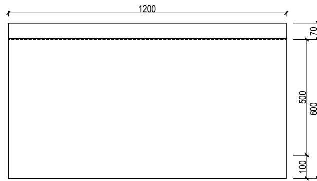
TAMPAK SAMPING U-DITCH
