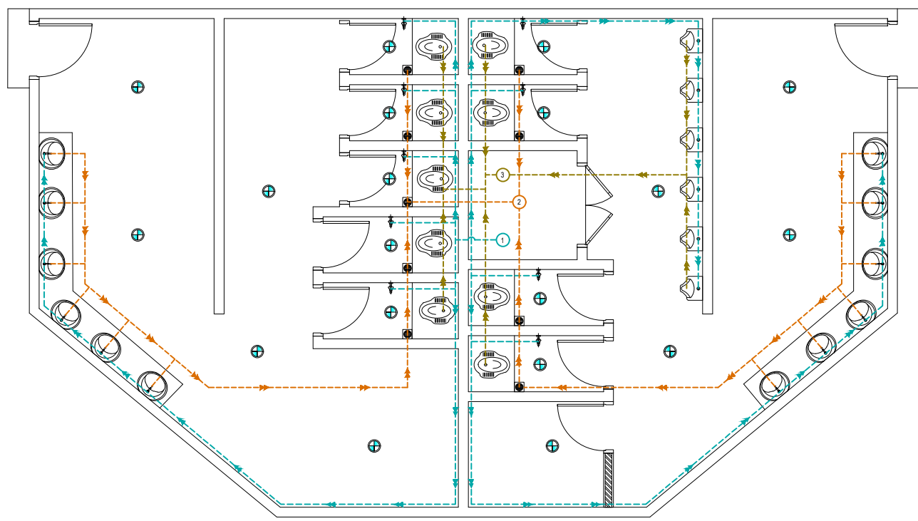
GSG ARS 1: 75 DENAH INSTALASI MEKANIKAL & ELEKTRIKAL
