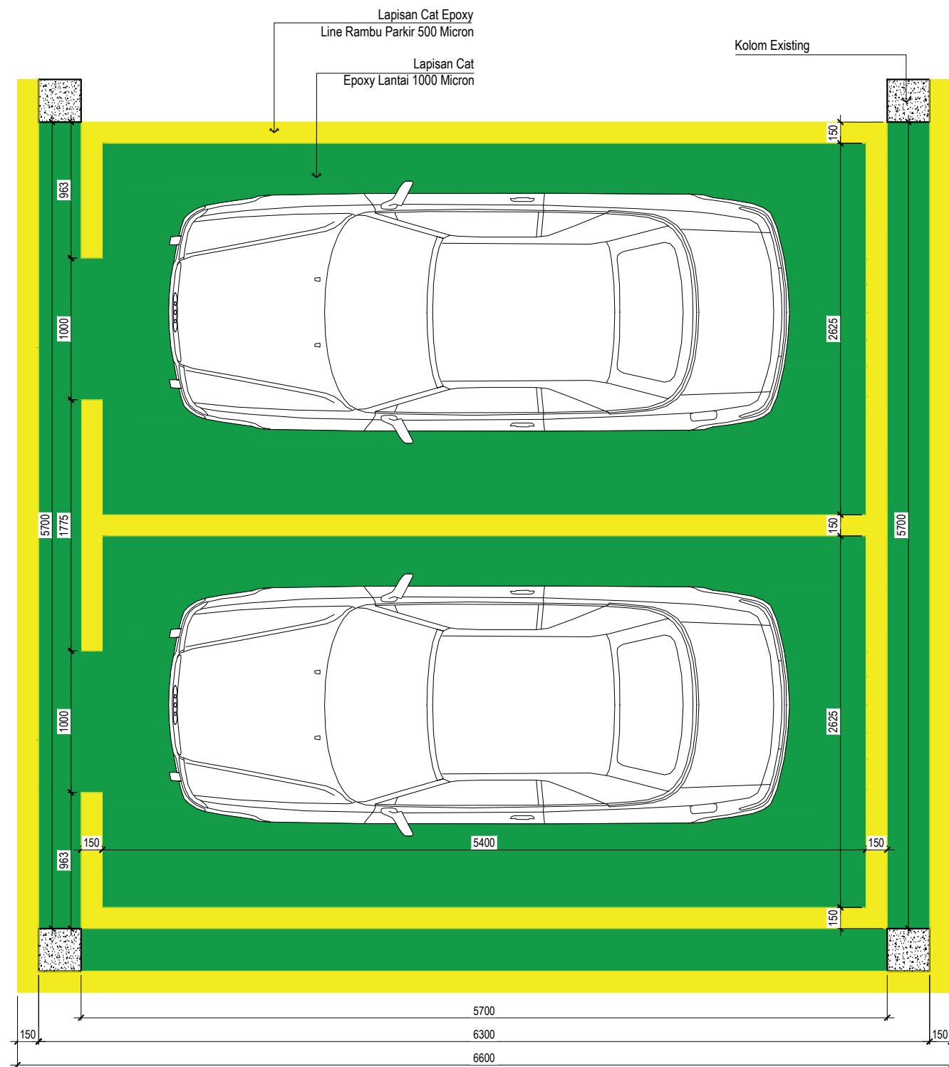
GSG ARS 1:35 DETAIL PENGECATAN RAMBU PARKIR RODA 4
