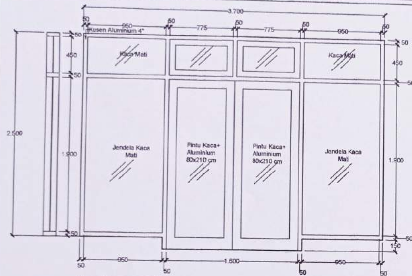
KUSEN P2J2 (3 UNIT) GEDUNG GIZI SKALA 1 : 30
