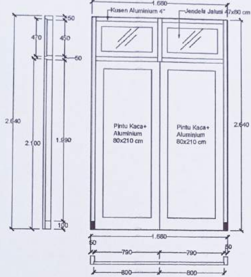
DETAIL KUSEN P2 (3 Unit)
