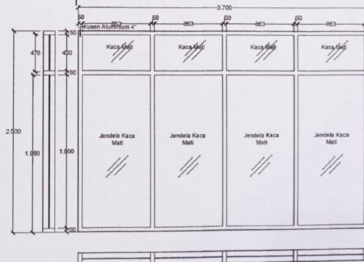
KUSEN P2 (3 UNIT) Rg. Apotek SKALA 1 : 30
