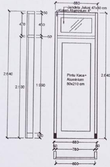
KUSEN P1 (6 UNIT) Rg. Apotek SKALA 1 : 30
