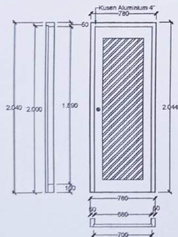
DETAIL KUSEN PA (1 Unit)
