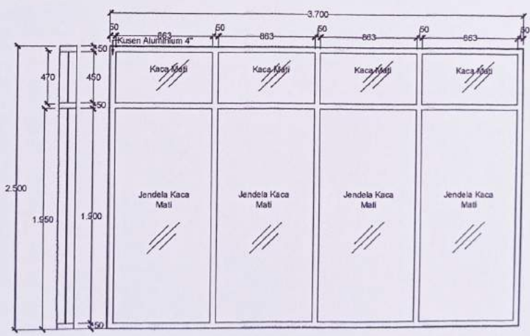
KUSEN J4 (2 UNIT) GEDUNG GIZI SKALA 1 : 30
