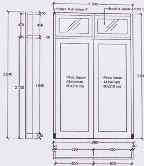
KUSEN P2 (3 UNIT) Rg. Apotek SKALA 1 : 30
