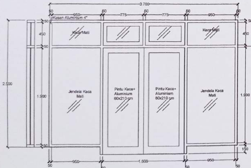
KUSEN P2.J2 (3 UNIT) Rg. Apotek SKALA 1 : 30
