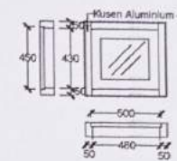
KUSEN V1 (2 UNIT) Rg. Apotek SKALA 1 : 30
