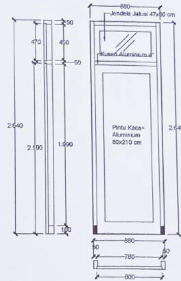
DETAIL KUSEN P1 (2 Unit)
