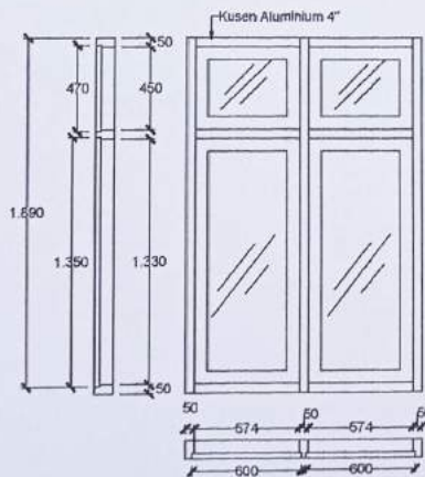
DETAIL KUSEN J2 (12 Unit)
