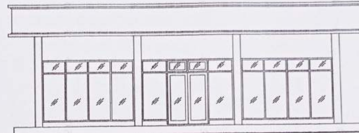
TAMPAK SAMPING KANAN Rg. Apotek SKALA 1 : 100
