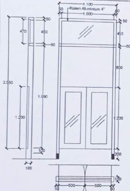
DETAIL KUSEN P2a(Koboy) (1 Unit)
