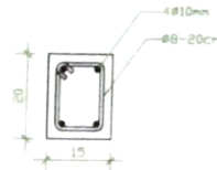
Detail Balok 20x15
