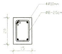
Detail Balok 20x15
