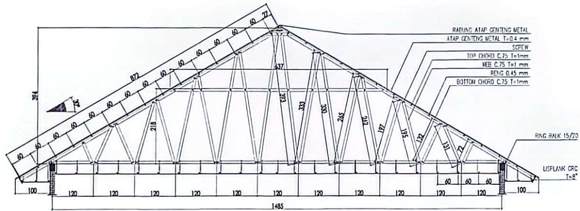
DETAIL POT. KUDA - KUDA (K2) SKALA 1:70
