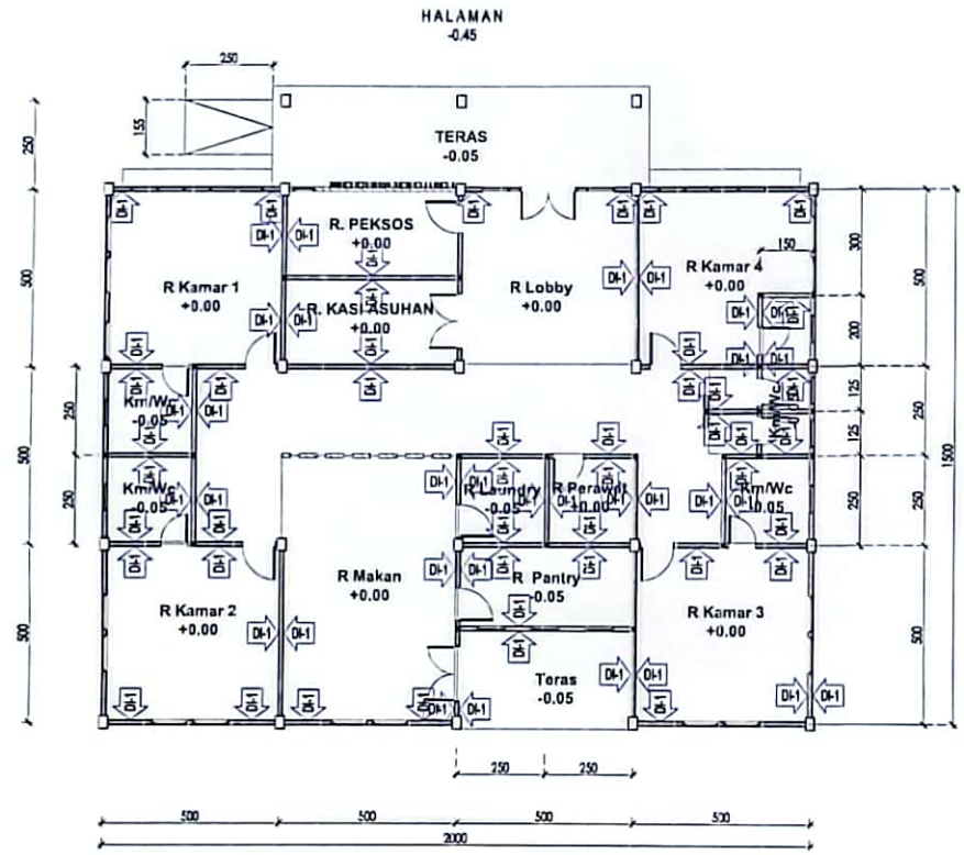
SKALA 1:150 DENAH RENC. FINISHING DINDING INTERIOR
