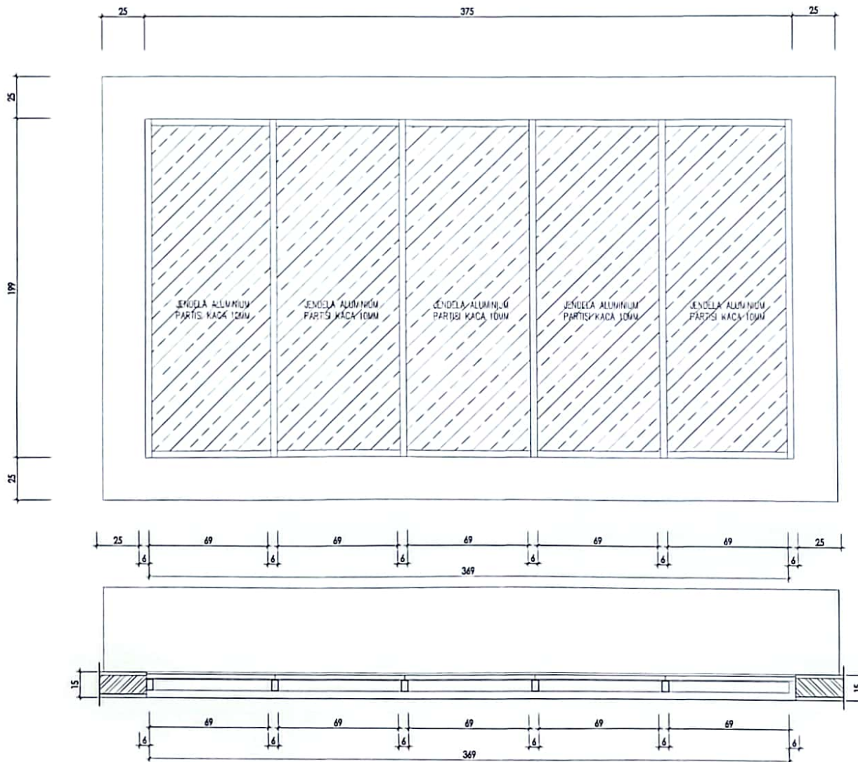
DETAIL JENDELA J1 = 2 UNIT SKALA 1:20
