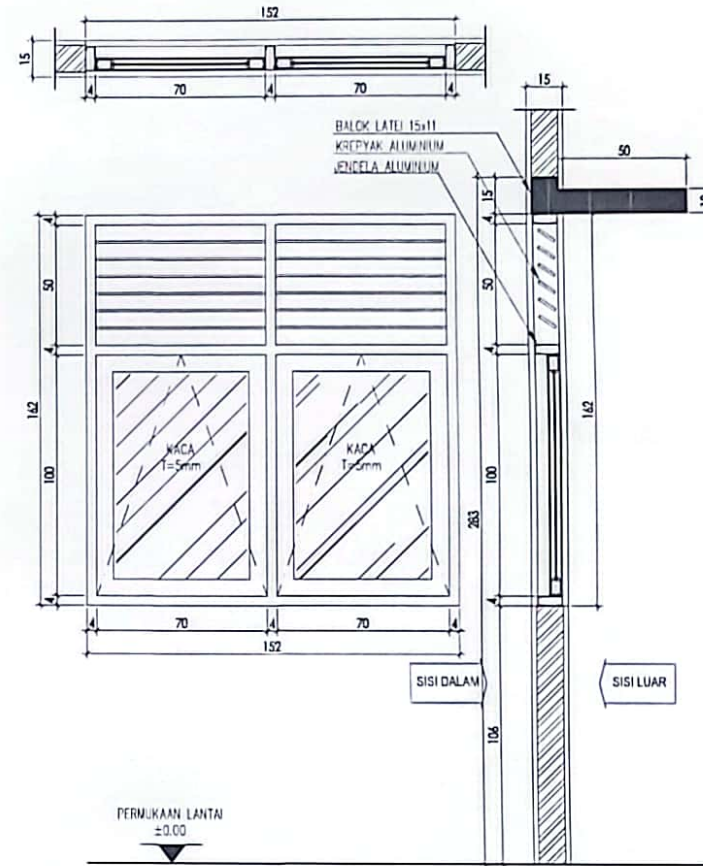
DETAIL JENDELA J2 = 7 UNIT SKALA 1:20
