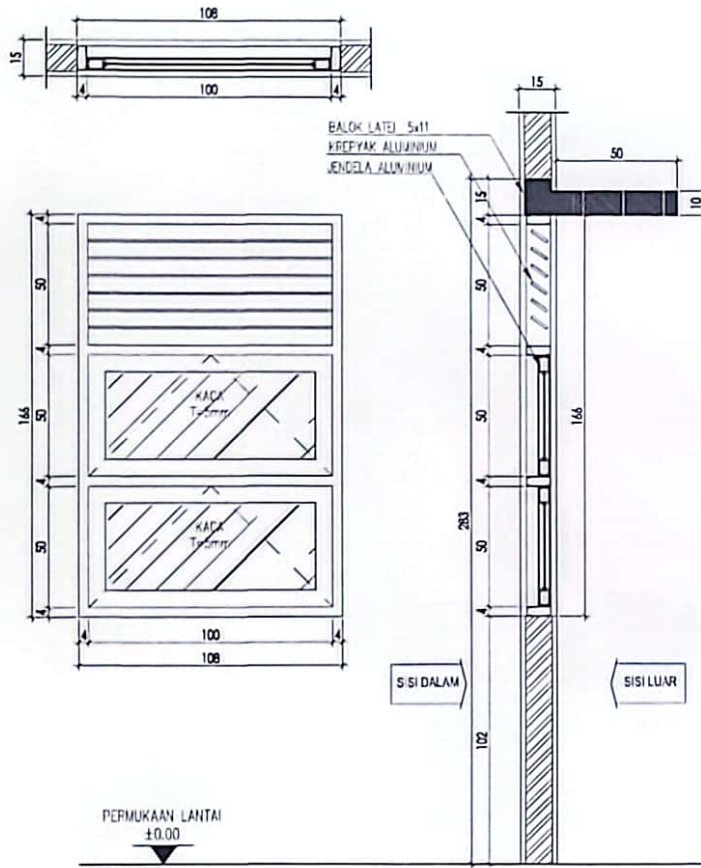
DETAIL JENDELA J2A = 15 UNIT SKALA 1:20
