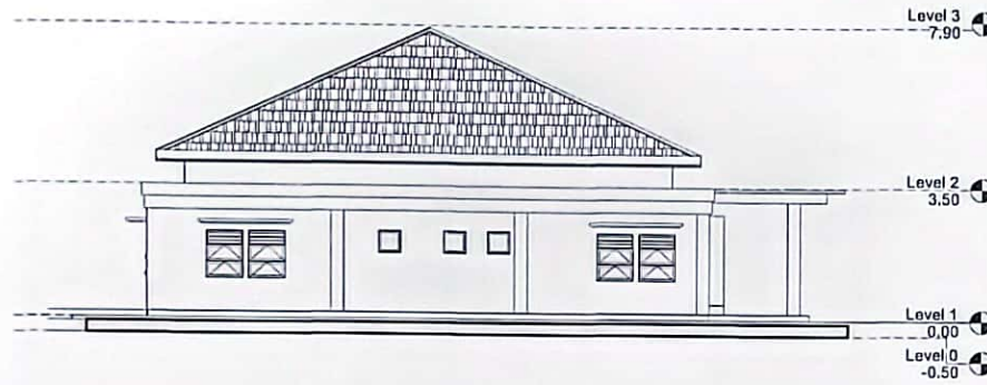
VIEW - C SKALA 1:150
