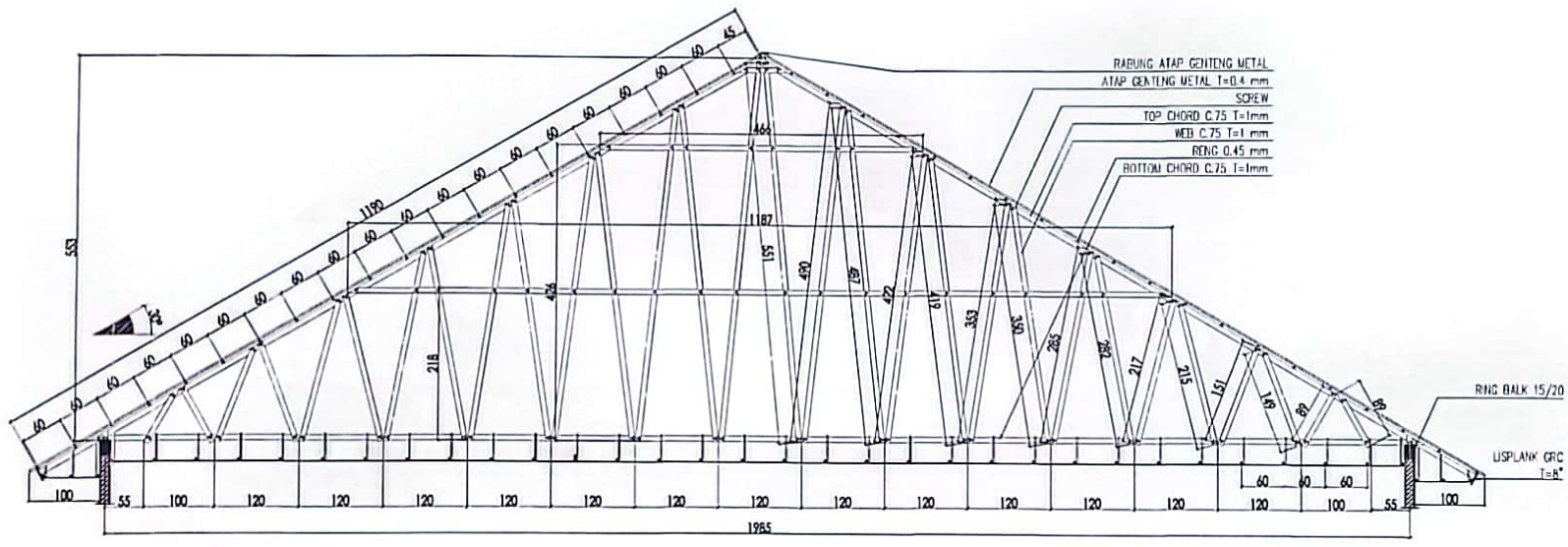
DETAIL POT. KUDA - KUDA (K1) SKALA 1:70
