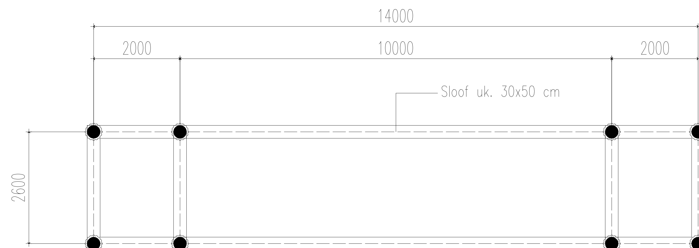
DENAH SLOOF SKALA 1:100
