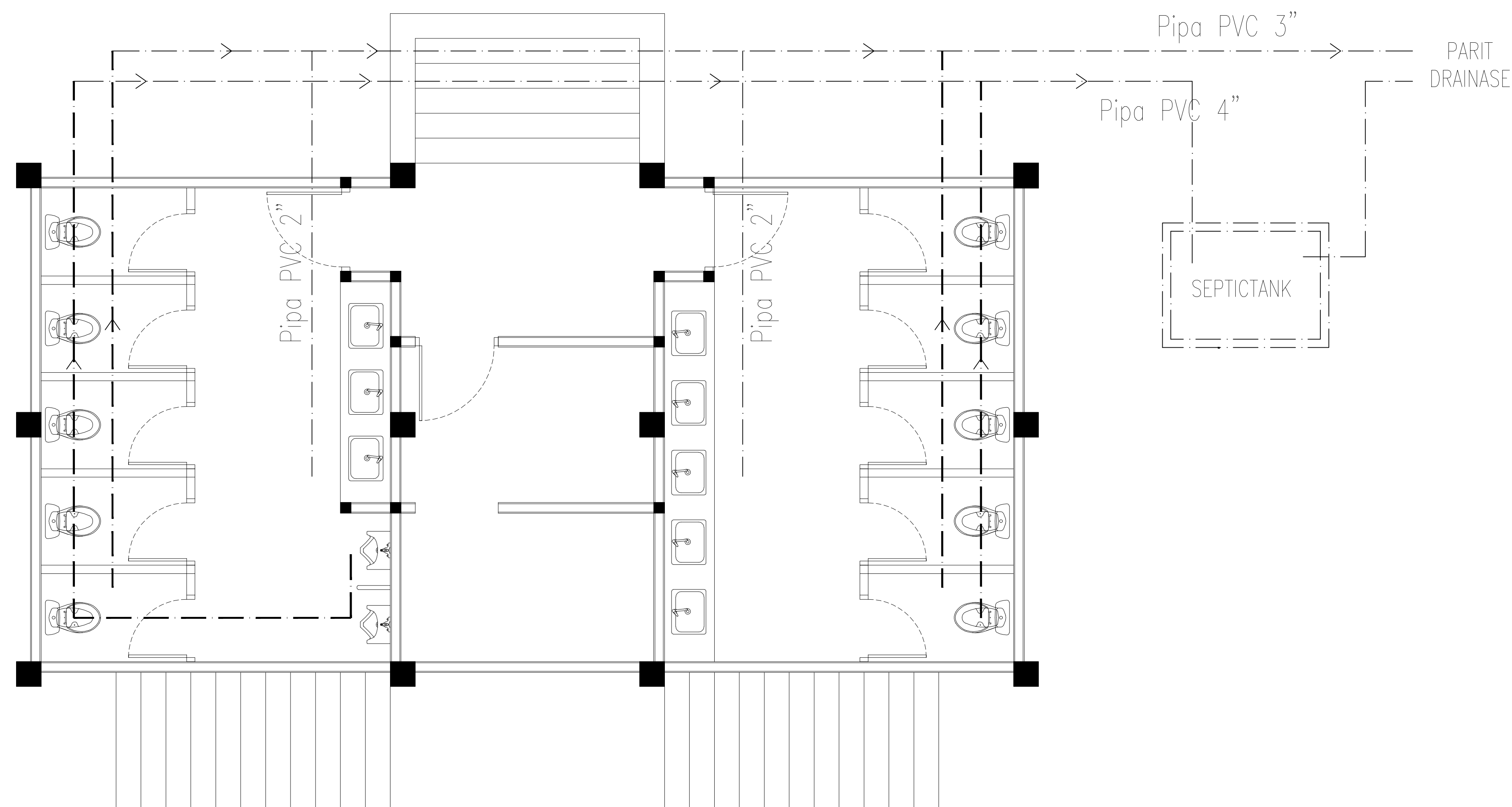
DENAH INSTALASI AIR KOTOR KAMAR MANDI SKALA 1:100
