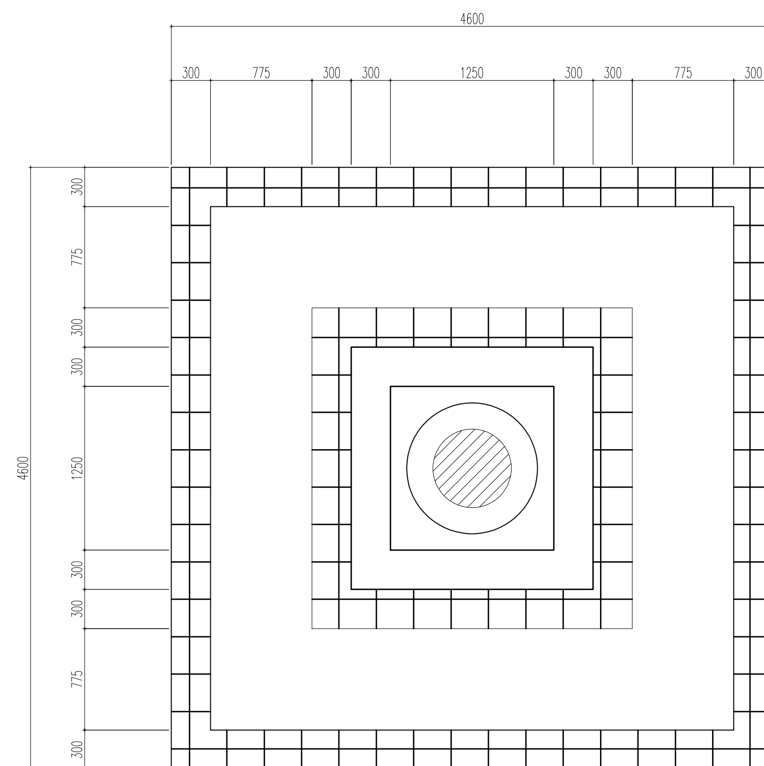
DENAH TUGU NOL EXISTING SKALA 1:100
