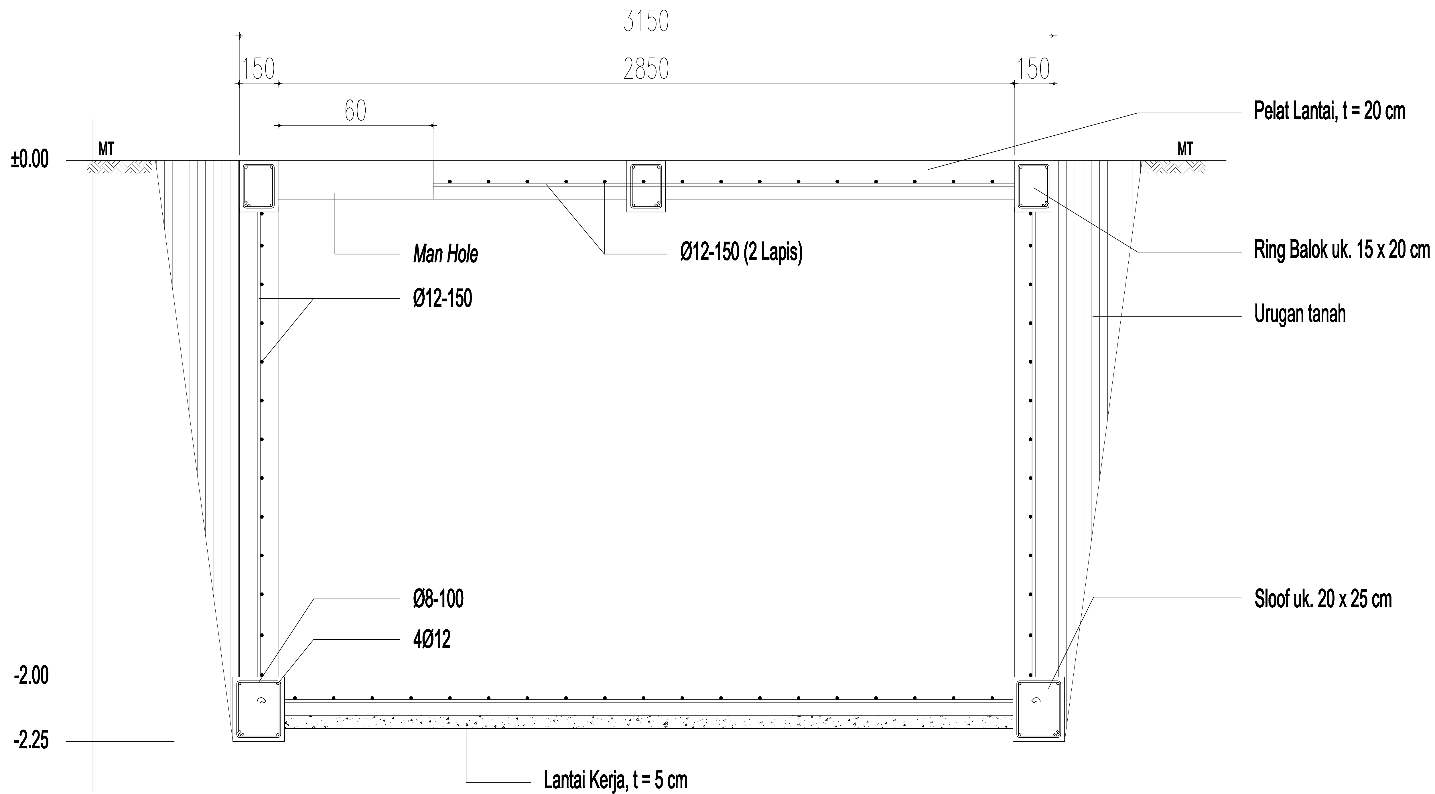
POTONGAN GROUND WATER TANK SKALA : NTS
