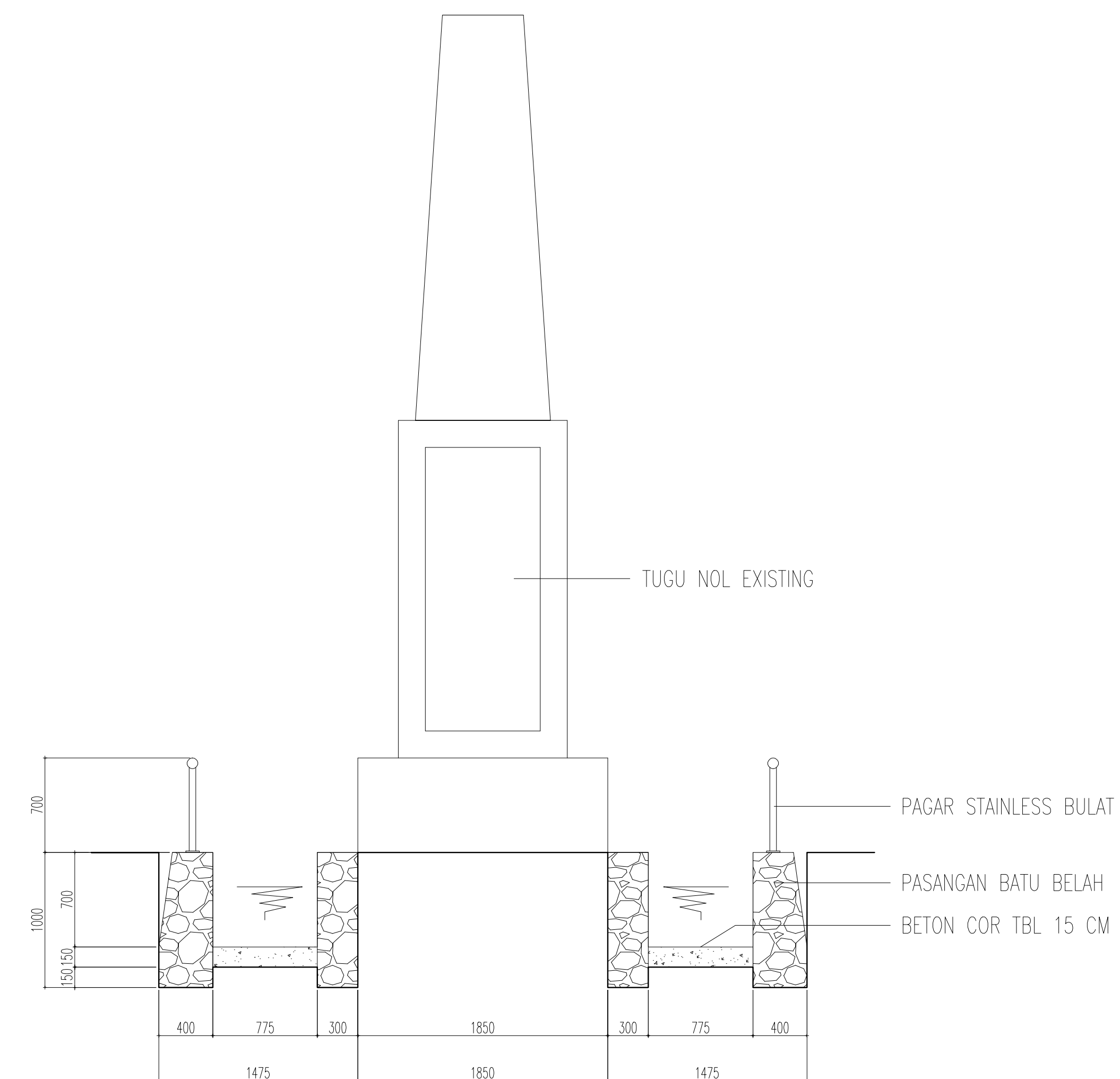
POTONGAN TUGU NOL EXISTING SKALA 1:100
