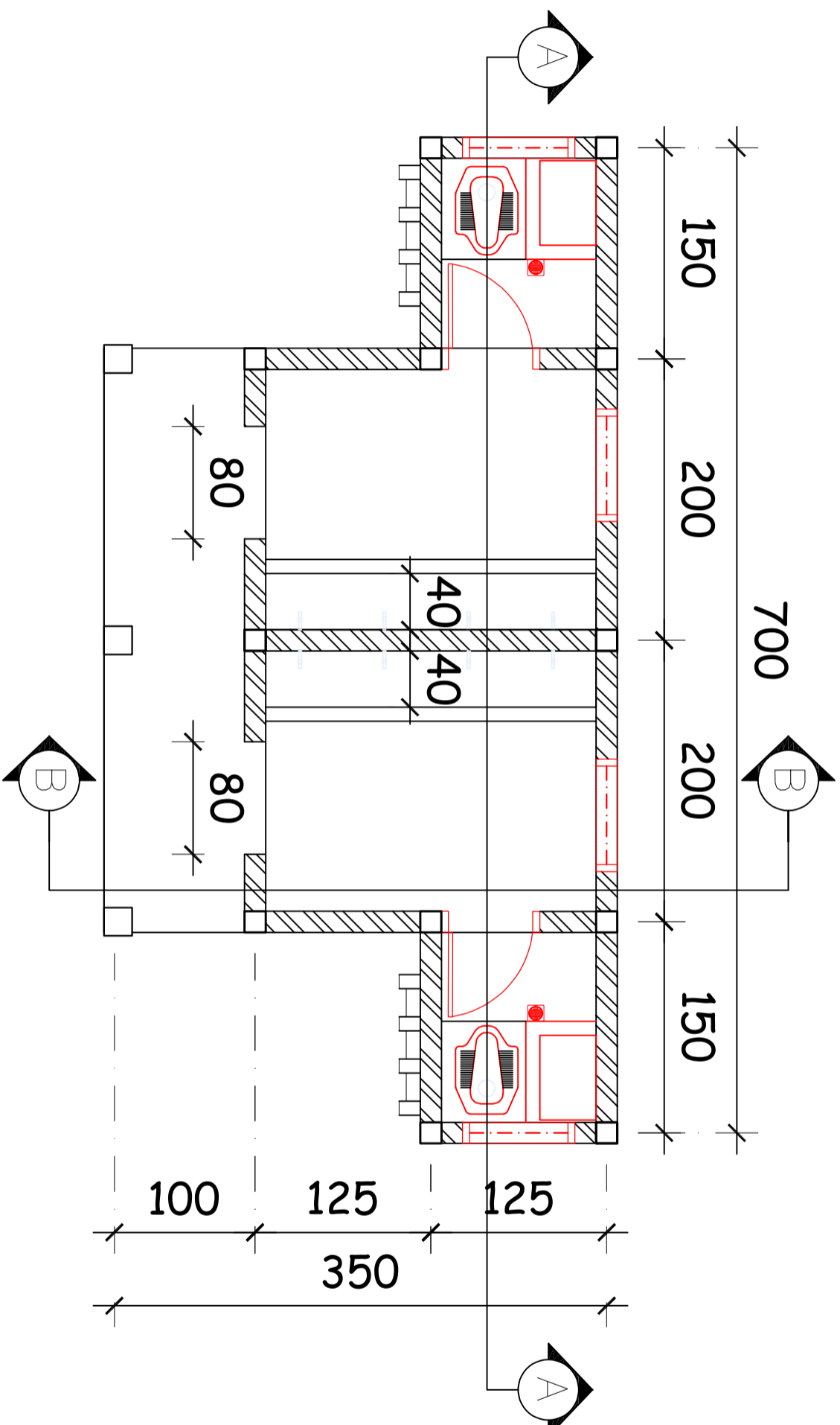
DENAH T. WUDHU SKALA 1:50
