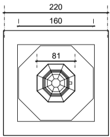
DENAH TIANG BENDERA (A) Skala 1 : 50
