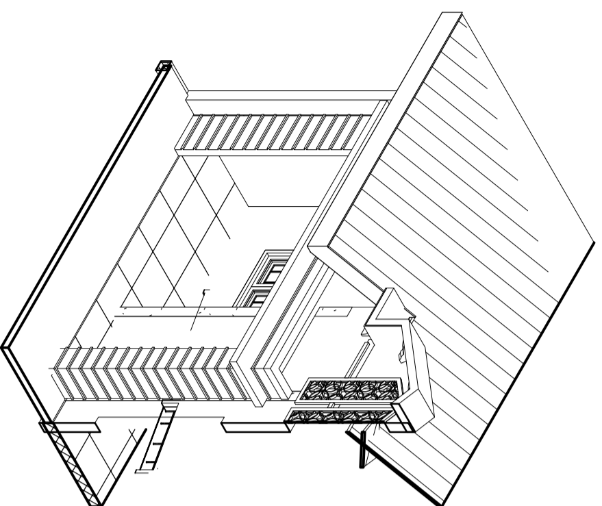
DENAH DETAIL 2
