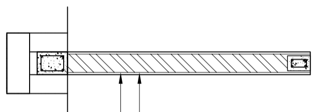
DETAIL RING BALOK RB1 SKALA 1:25
