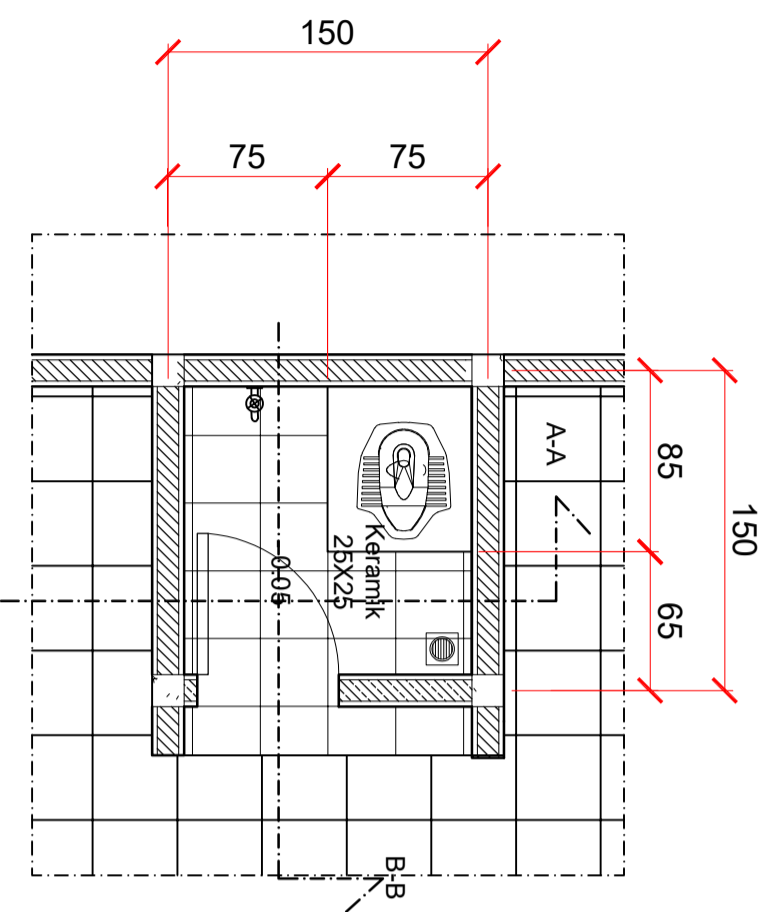
DETAIL KAMAR MANDI SKALA 1:20
