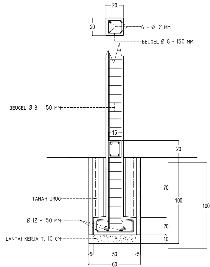
DETAIL PONDASI TAPAK SELASAR SKALA 1: 25
