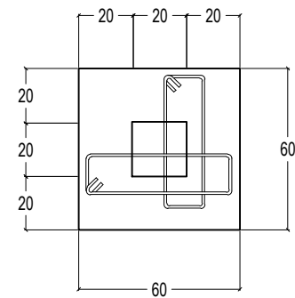
DENAH PONDASI TAPAK SKALA 1: 25
