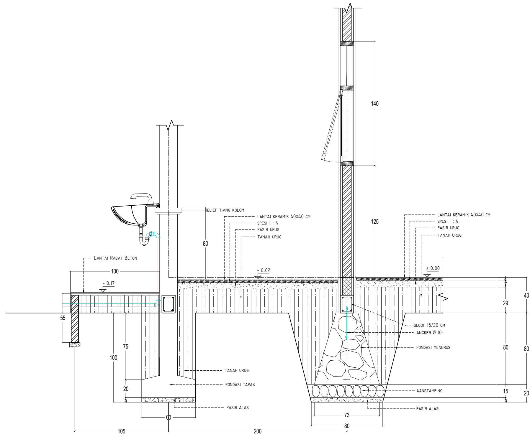
DETAIL 1-1 SKALA 1: 25
